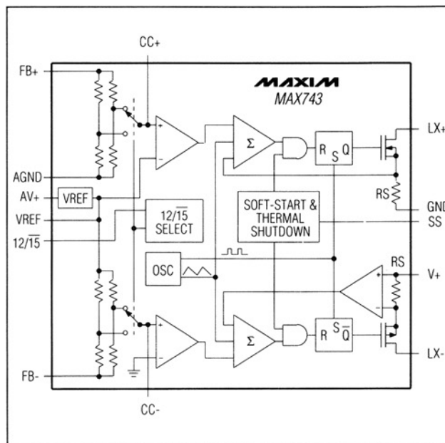
Figure 3. MAX743 Block Diagram
