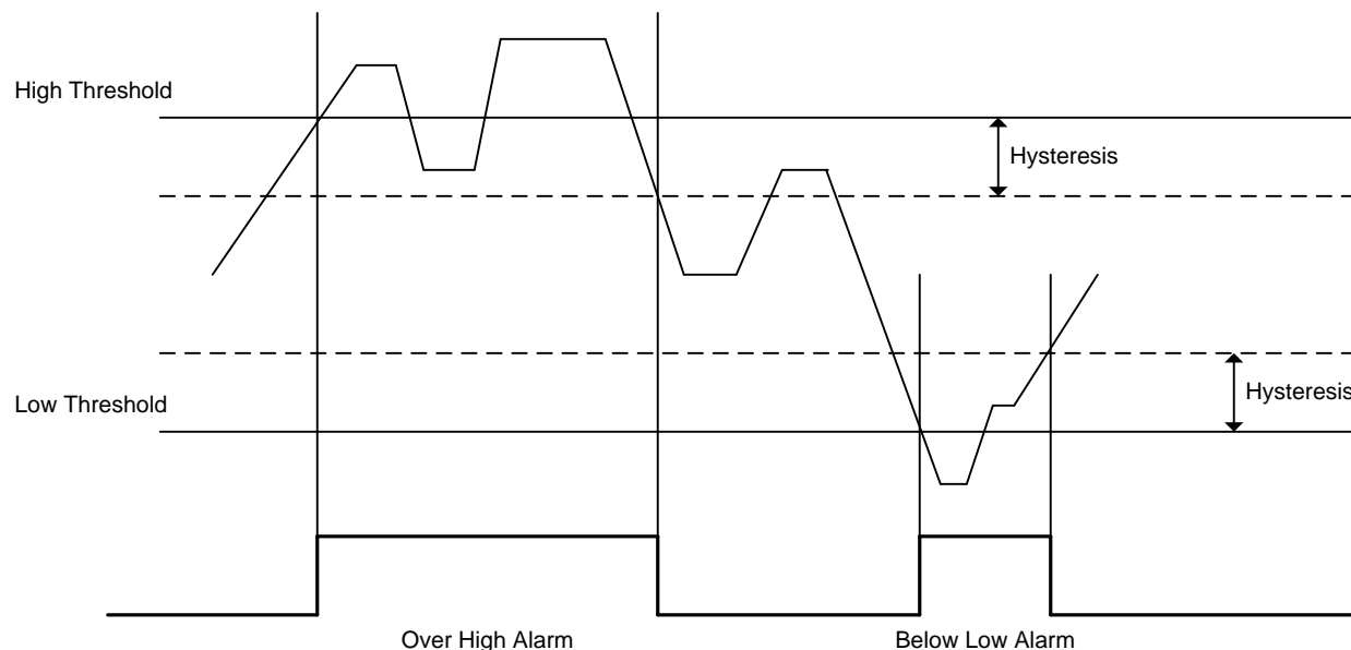
Figure 50. AMC7832 Hysteresis
