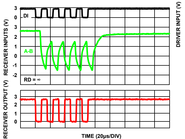
FIGURE 15. ISL32600E, ISL32601E PERFORMANCE WITH V_{CC} = 2.7V , 128kbps, 4000ft (1220m) CAT 5 CABLE
