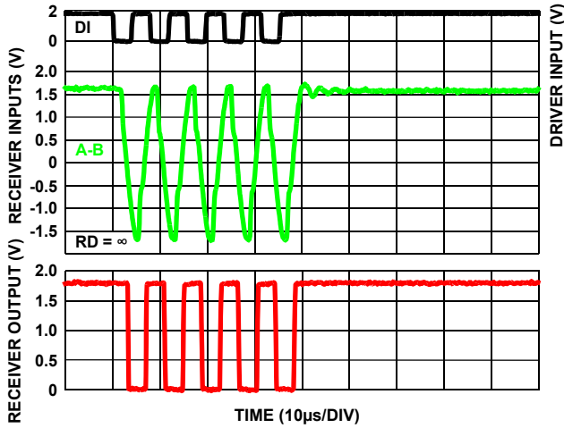
FIGURE 28. ISL32602E, ISL32603E PERFORMANCE WITH V_{CC} = 1.8V , 256kbps, 1000ft (305m) CAT 5 CABLE
