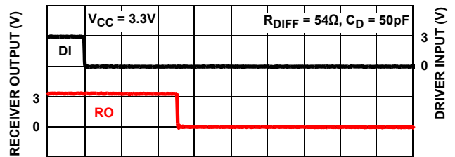
FIGURE 35. ISL32602E, ISL32603E DRIVER AND RECEIVER WAVEFORMS, HIGH TO LOW
