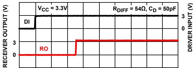
FIGURE 34. ISL32602E, ISL32603E DRIVER AND RECEIVER WAVEFORMS, LOW TO HIGH
