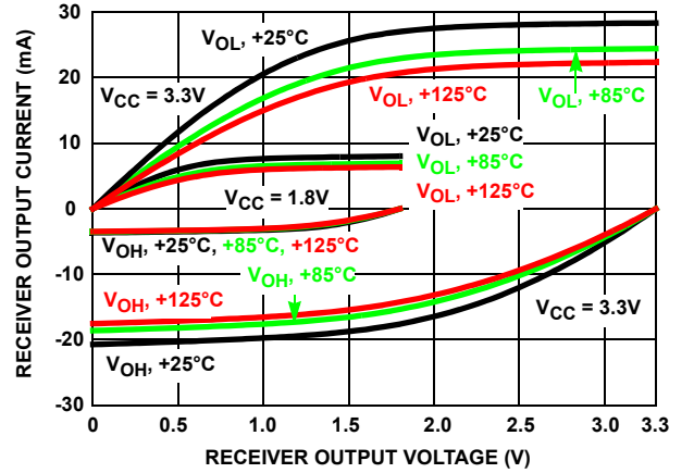
FIGURE 25. ISL32602E, ISL32603E RECEIVER OUTPUT CURRENT vs RECEIVER OUTPUT VOLTAGE
