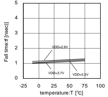
Fig.51 24.375MHz Fall-time temperature characteristics
