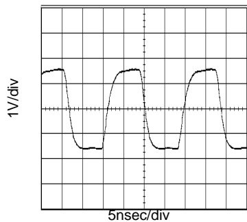
Fig.1 54MHz output waveform (VDD=3.3V, CL=15pF, Ta=25°C)
