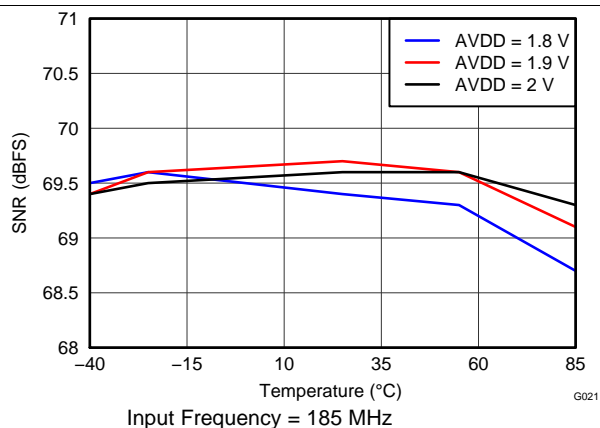
Figure 23. Signal-to-Noise Ratio vs AVDD Supply and Temperature
