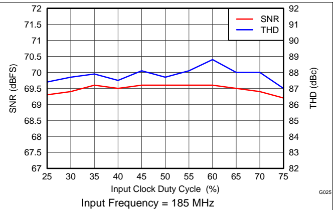
Figure 27. Performance vs Clock Duty Cycle
