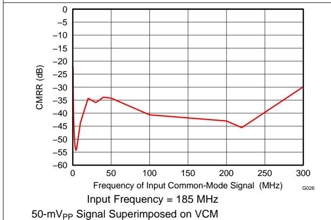
Figure 28. Common-Mode Rejection Ratio Spectrum
