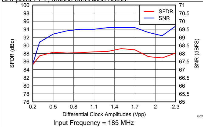
Figure 26. Performance vs Clock Amplitude
