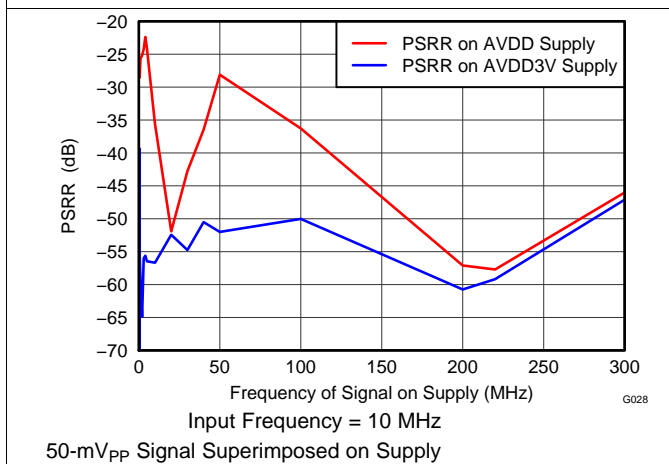
Figure 30. Power-Supply Rejection Ratio Spectrum for AVDD
