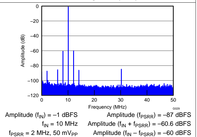
Figure 31. Power-Supply Rejection Ratio vs Test Signal Frequency
