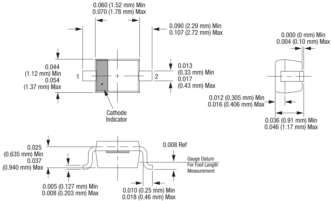
Figure 9. SOD-323 Package Dimension Drawing
