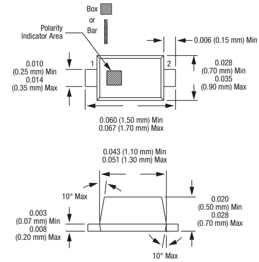
Dimensions are in inches (millimeters shown in parentheses) 200043-007
