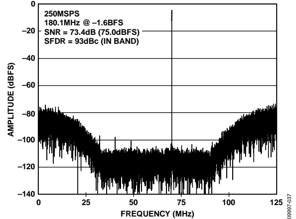
Figure 37. 22% Bandwidth Mode, Tuning Word = 28
