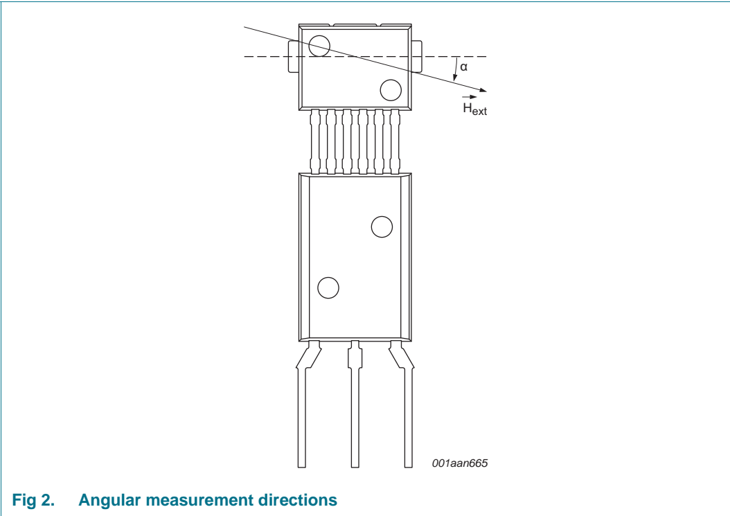
Fig 2. Angular measurement directions Since the Anisotropic MR (AMR) effect is periodic over 180°, the sensor output is also 180°-periodic, where the angle is calculated relative to a freely programmable zero angle. The dashed line indicates the mechanical zero degree position.
