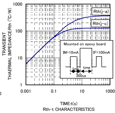
Rth-t CHARACTERISTICS
