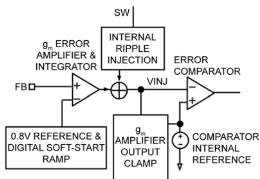
Figure 10. Internal Ripple Injection
