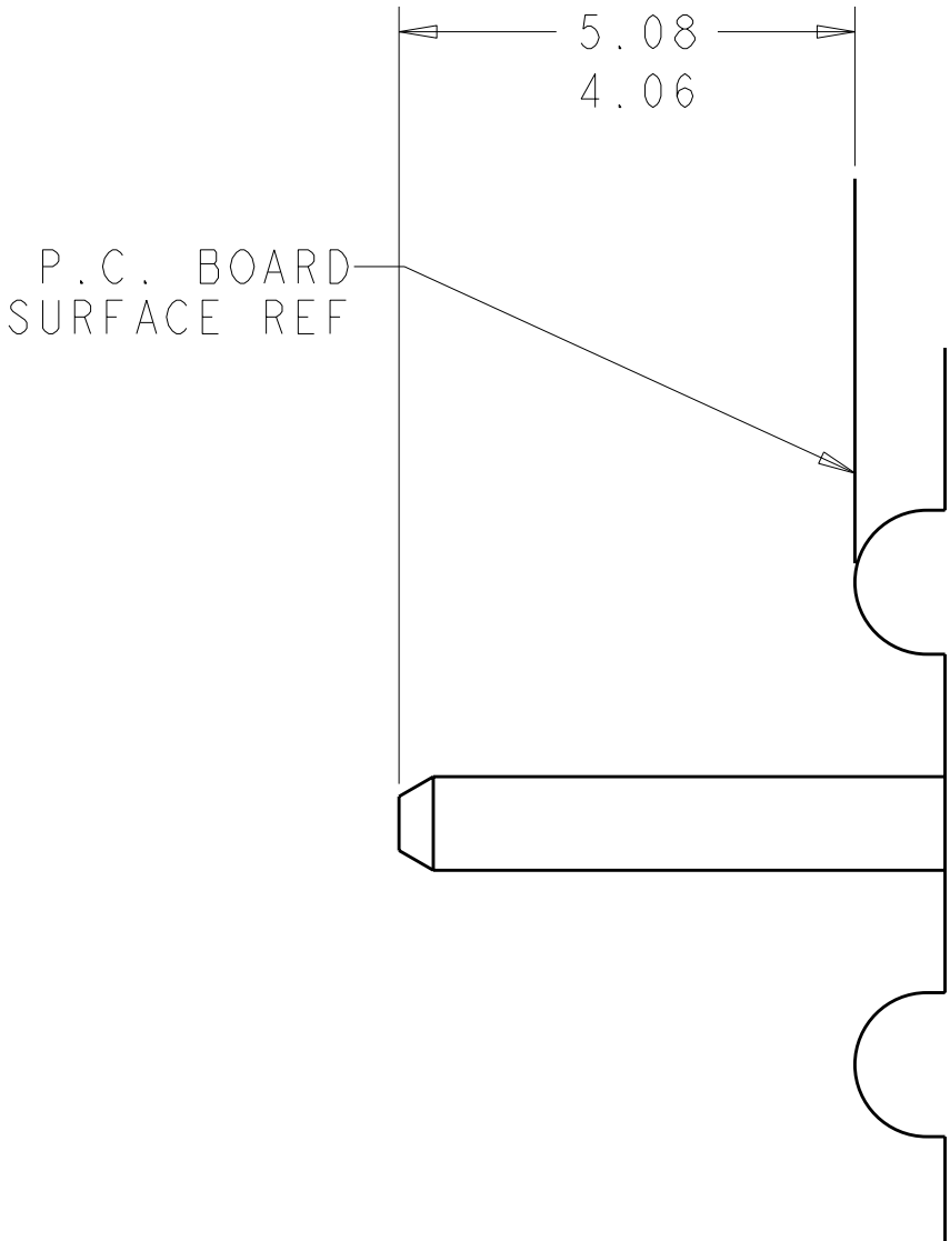
5. SOLDER TAIL DETAIL SCALE 10 : 1
