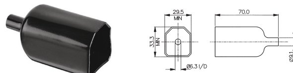
Insulation Boot
