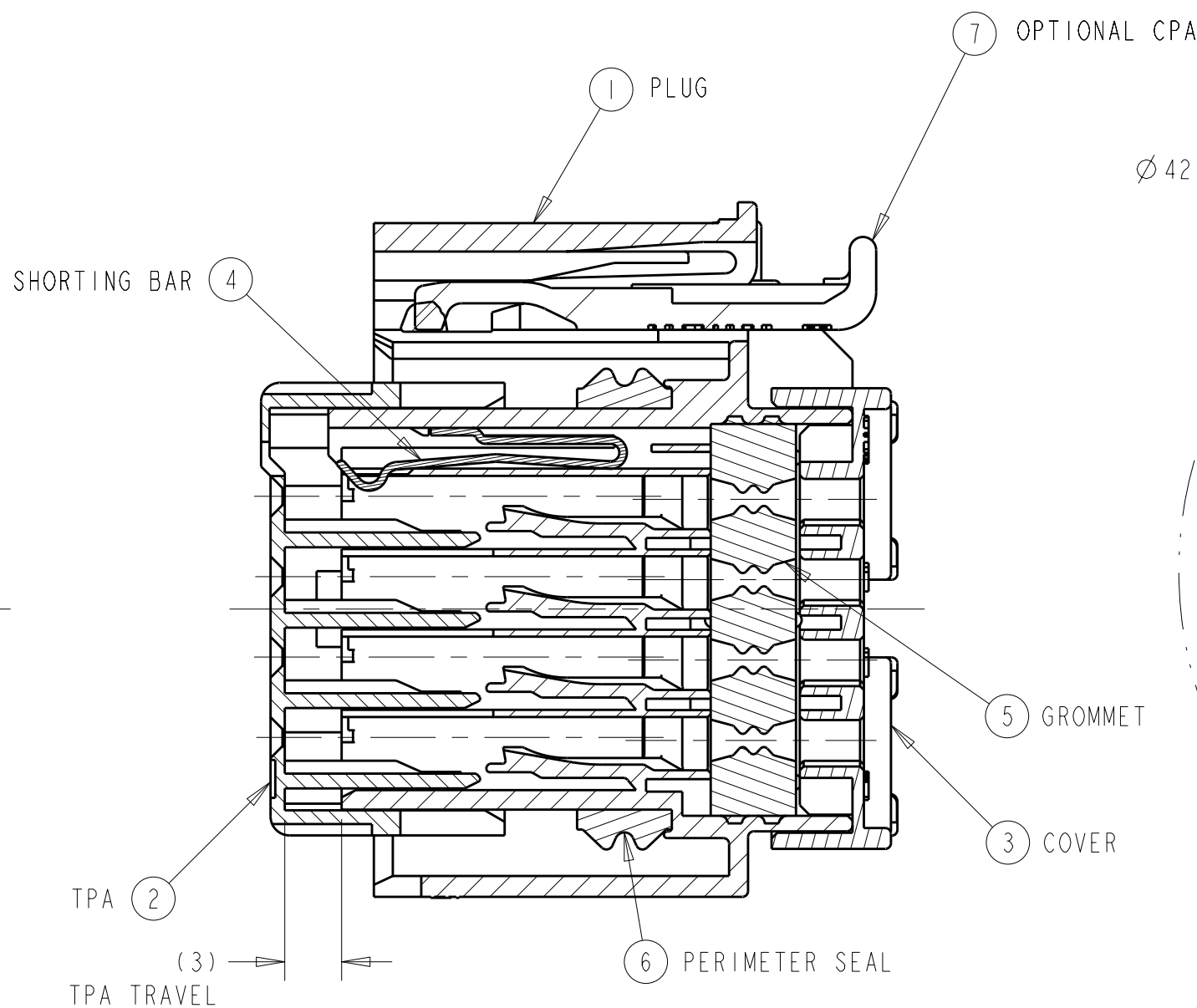
SECTION A-A SHOWN WITH TPA IN IT'S PRE-LOADED POSITION (DELIVERY CONDNTION)
