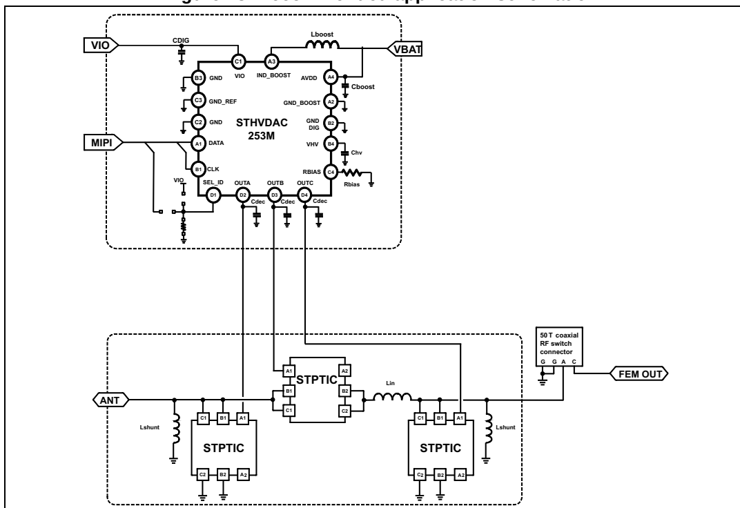
Figure 14. Evaluation board
