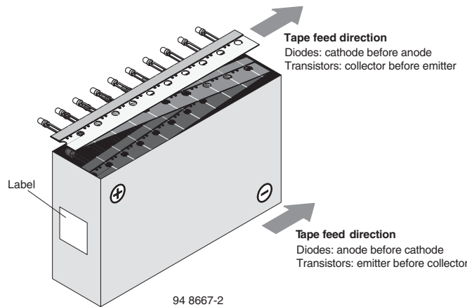
Fig. 26 - Tape Direction
