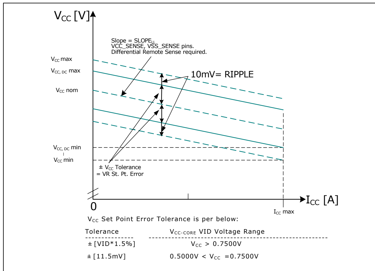
Figure 14. Active V_{CC} and I_{CC} Loadline (PSI# Not Asserted)
