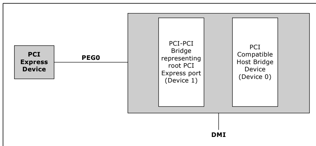
Figure 6. PCI Express Related Register Structures
