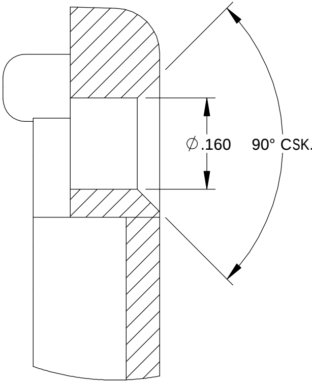
DETAIL D SCALE 6 : 1
