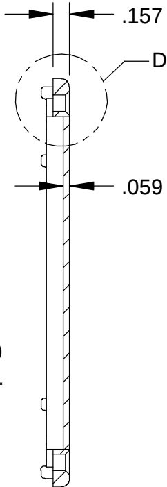
SECTION C-C
