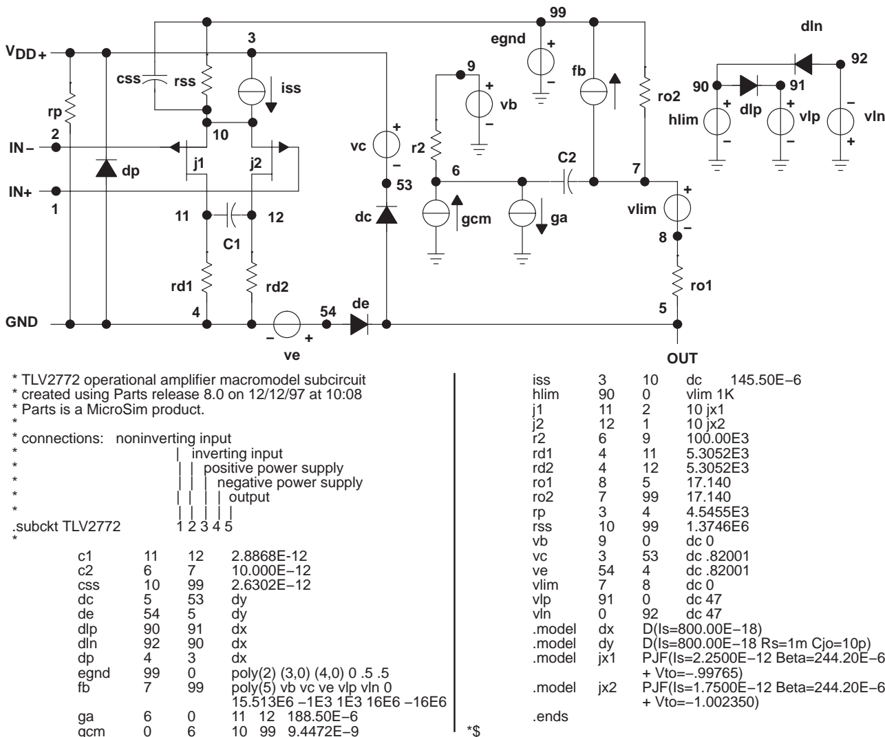
Figure 64. Boyle Macromodel and Subcircuit
