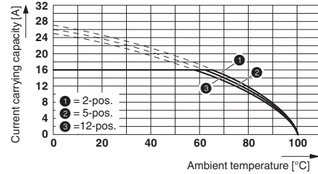
Derating curve for: GIC 2,5 HC/...-ST-7,62 with GIC 2,5 HC/...-G-7,62
