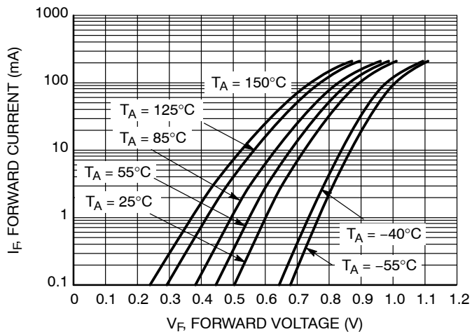
Figure 12. Forward Voltage
