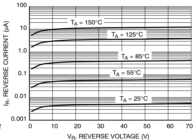
Figure 13. Leakage Current
