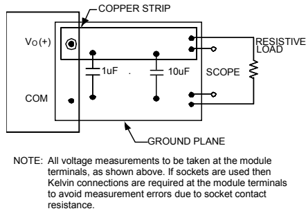
Figure 38. Output Ripple and Noise Test Setup.
