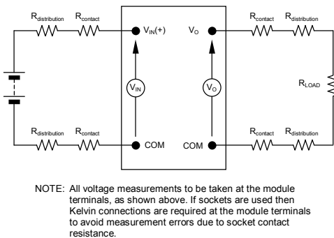
Figure 39. Output Voltage and Efficiency Test Setup.
