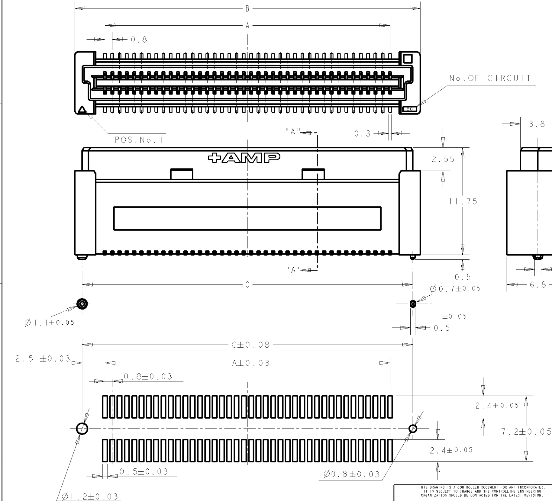
RECOMMENDED P.C.BOARD LAYOUT
