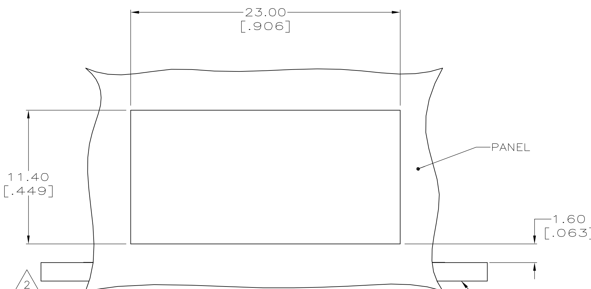
RECOMMENDED PANEL CUTOUT SCALE 5:1
