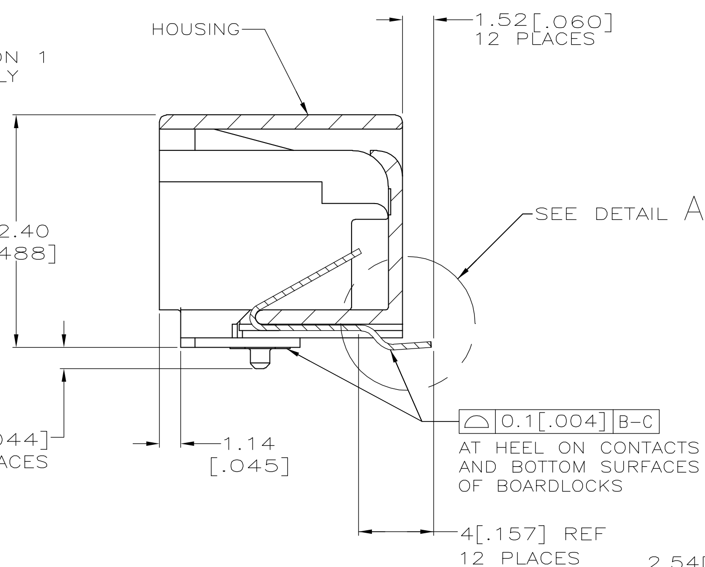
SECTION C-C
