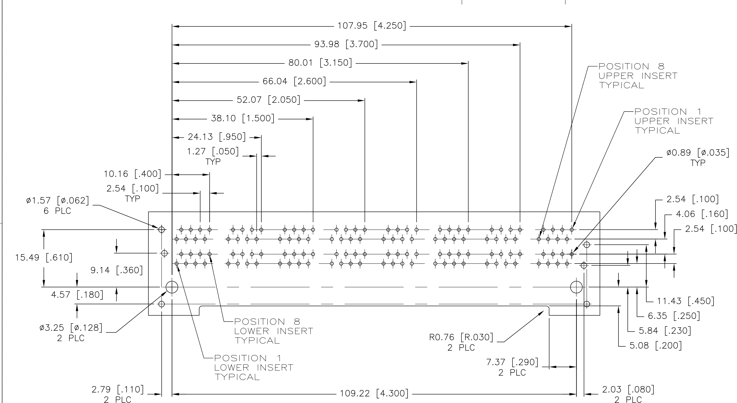
PC BOARD LAYOUT VIEWED FROM COMPONENT SIDE SCALE 2:1
