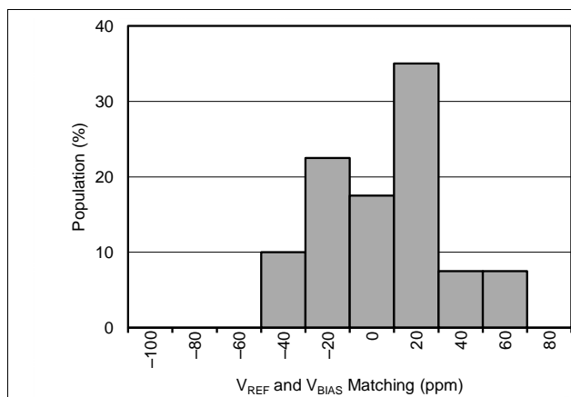
Figure 48. V_{REF} - 2 \times V_{BIAS} Distribution (At T_A = 25^\circ\text{C} )
