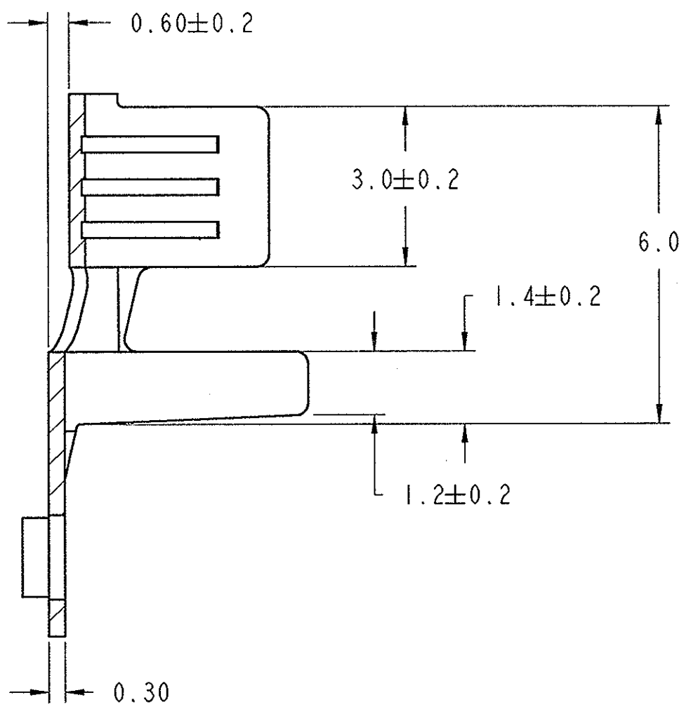
SECTION C-C
