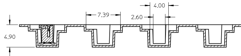
SECTION Z-Z
