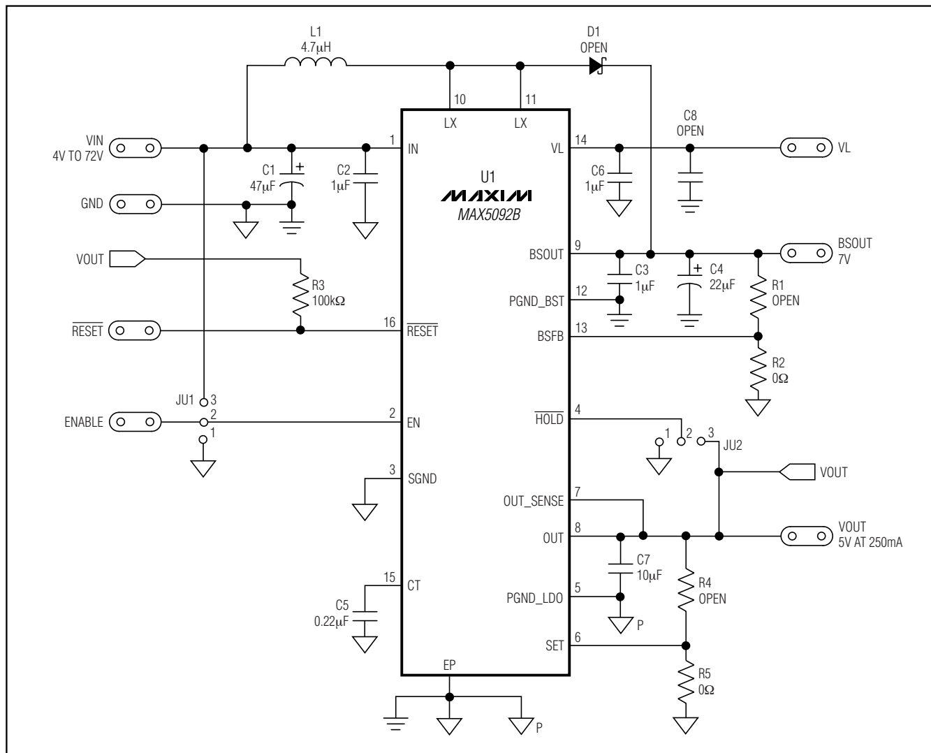
Figure 2. MAX5092B EV Kit Schematic
