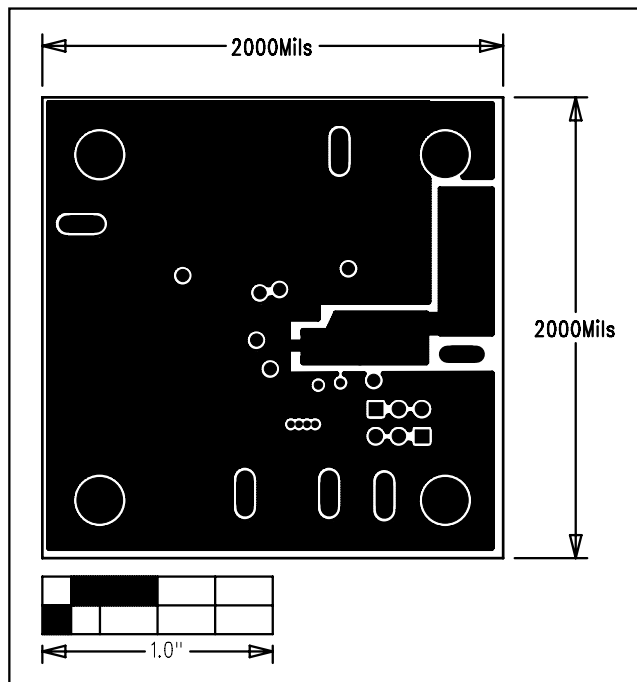
Figure 7. MAX5092 EV Kit PCB Layout—Solder Side Bottom
