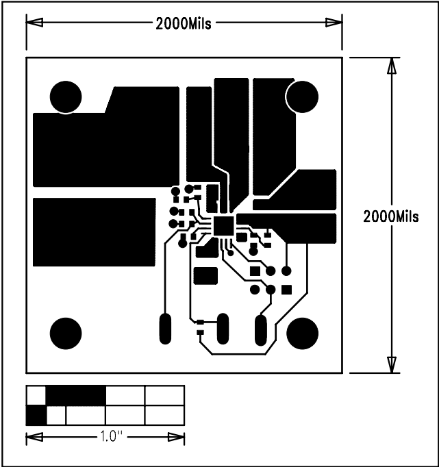
Figure 4. MAX5092 EV Kit PCB Layout—Solder Side Top
