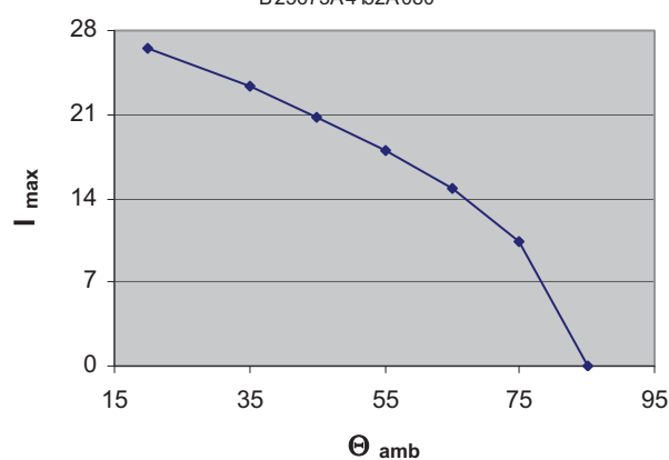
Max. allowable current (rms) at specific ambient Temp. B25673A4152A080
