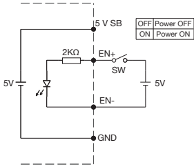
(C) Using external voltage source
