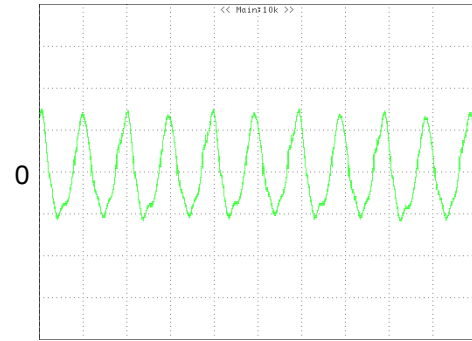
Figure 11: Input Terminal Ripple Current, i_c , at full rated output current and nominal input voltage with 12 \mu H source impedance and 100 \mu F electrolytic capacitor (100 mV/div, 2 \mu s/div)
