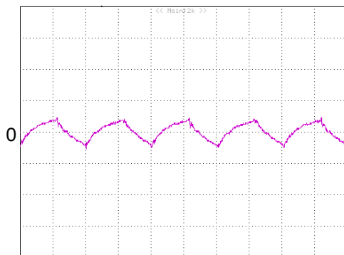
Figure 14: Output voltage ripple at nominal input voltage and rated load current ( I_o=40 A) (100 mV/div, 1 \mu s/div)
