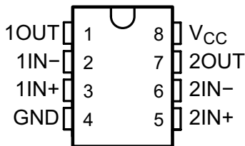
D, DGK, JG, P, PS, DDF or PW Package 8-Pin SOIC, VSSOP, PDIP, SO, or TSSOP Top View
