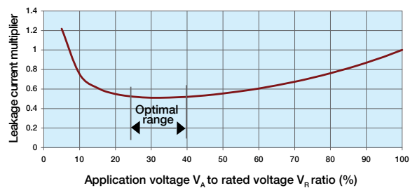
LEAKAGE CURRENT MULTIPLIER vs. VOLTAGE DERATING for FIXED APPLICATION VOLTAGE V_A
