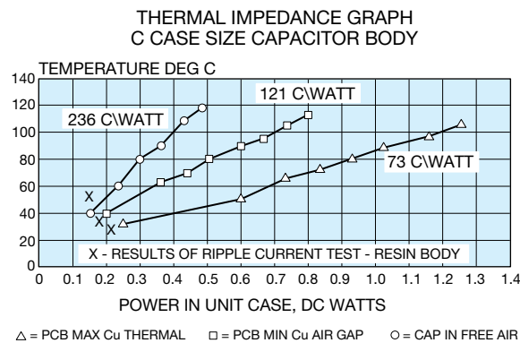
Thermal Impedance Graph with Ripple Current
