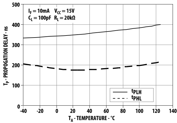
Figure 8. Propagation Delay with External 20\text{ k}\Omega R_L vs. Temperature.
