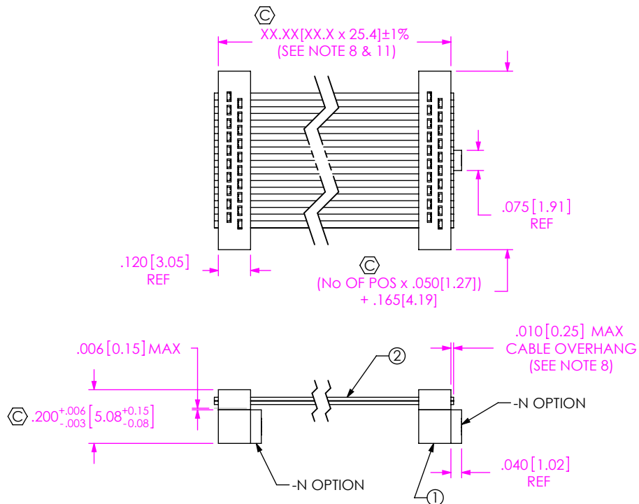
FIG 1 (FFSD-10-D-XX.XX-01-X-N SHOWN)
