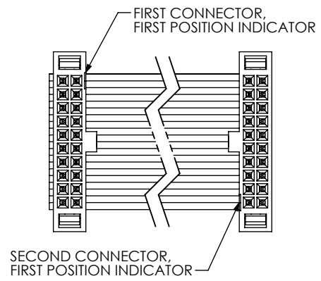
(FFSD-10-D-XX.XX-01-X-N-RN2 SHOWN) (SAME AS FIG 1, DIFFERENT AS SHOWN)
