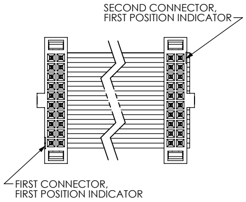
(FFSD-10-D-XX.XX-01-X-N-RN1 SHOWN) (SAME AS FIG 1, DIFFERENT AS SHOWN)
