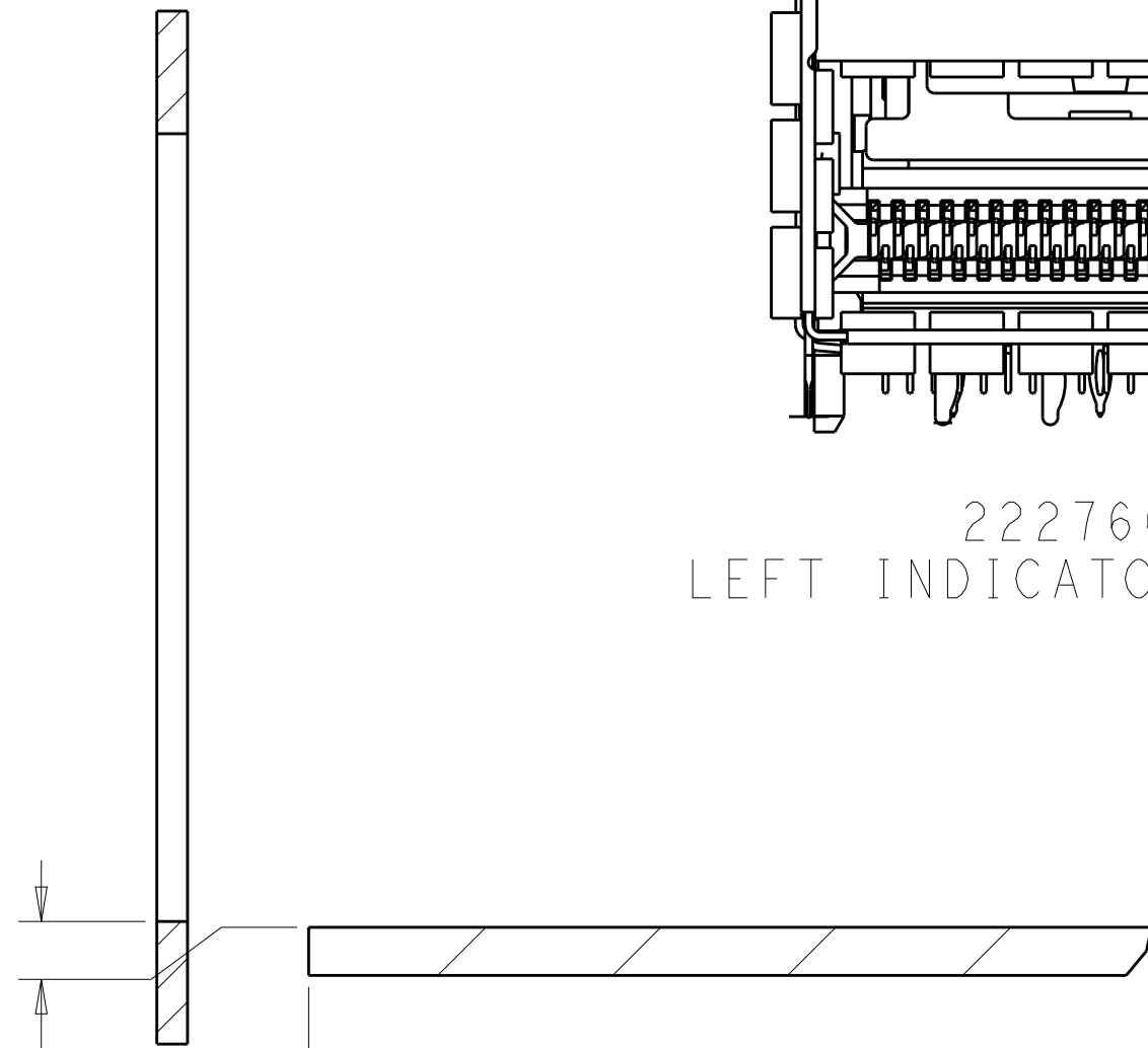
SECTION U-U
