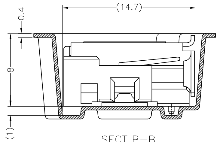
SECT B-B (4:1)
