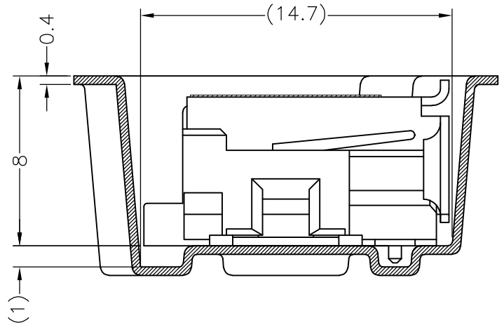
SECT B-B (4:1)
