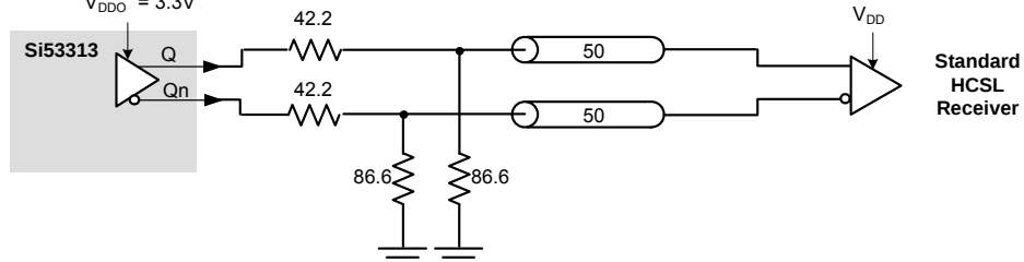
Figure 9. LVDS, CML, HCSL, and Low-Power LVPECL Output Termination
