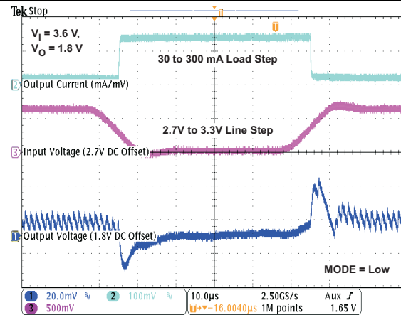
Figure 30. Combined Line/Load Transient Response
