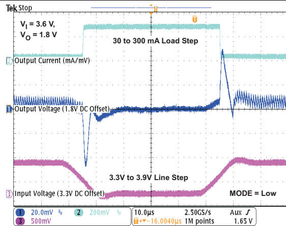
Figure 29. Combined Line/Load Transient Response
