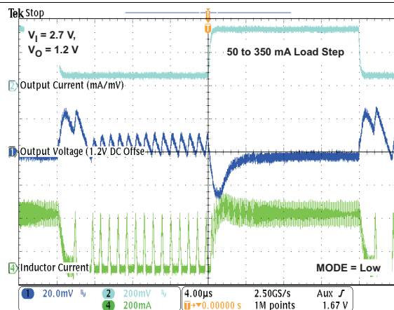
Figure 33. Load Transient Response in PFM/PWM Operation
