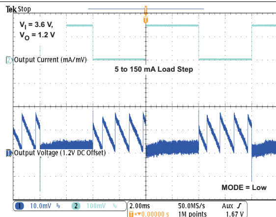
Figure 31. Load Transient Response in PFM/PWM Operation
