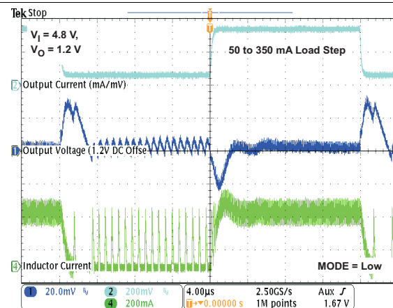
Figure 34. Load Transient Response in PFM/PWM Operation
