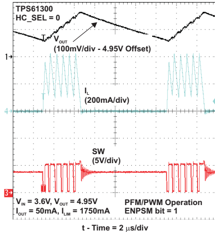
Figure 94. PFM Operation
