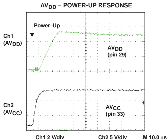
Figure 37. Power-Up Response
