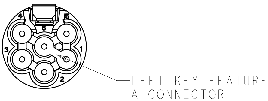
CONNECTOR A FROM VIEW A-A SCALE 2:1
