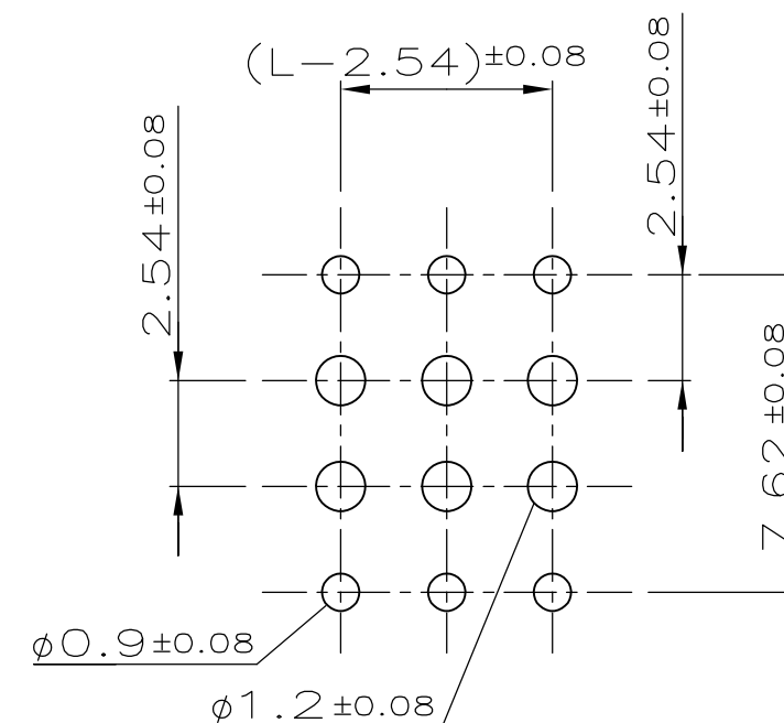
P.C.-BOARD HOLE-PATTERN
