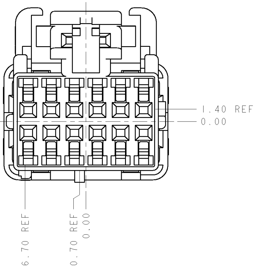
KEY CODE "D" (APPLIES TO -4 AND -8 ONLY) SCALE 4:1
