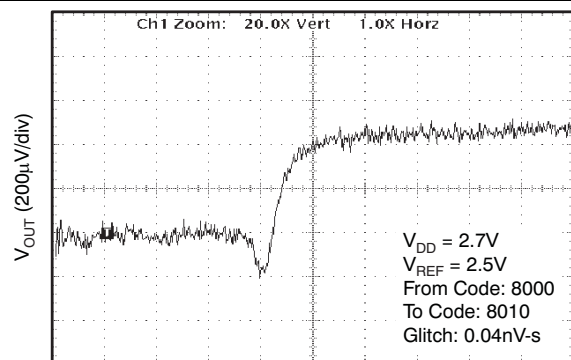
Time (400ns/div) 2.7 V 16-LSB Step
