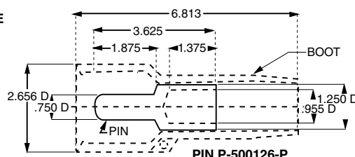
PIN P-500126-P
