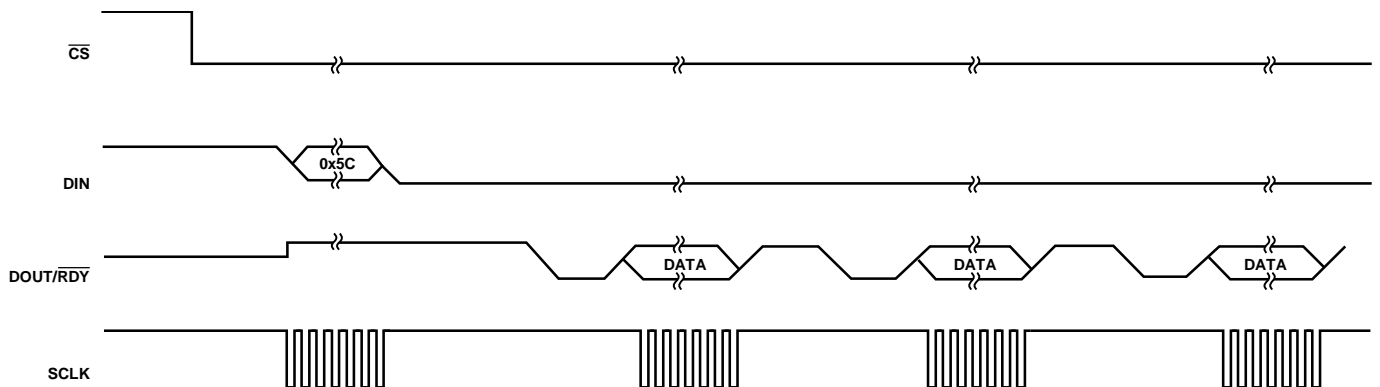
Figure 27. Continuous Read
