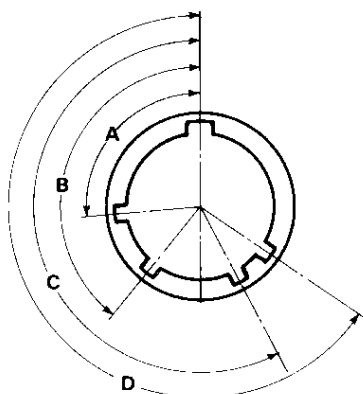
Vue face avant embase Viewed from face of receptacle
