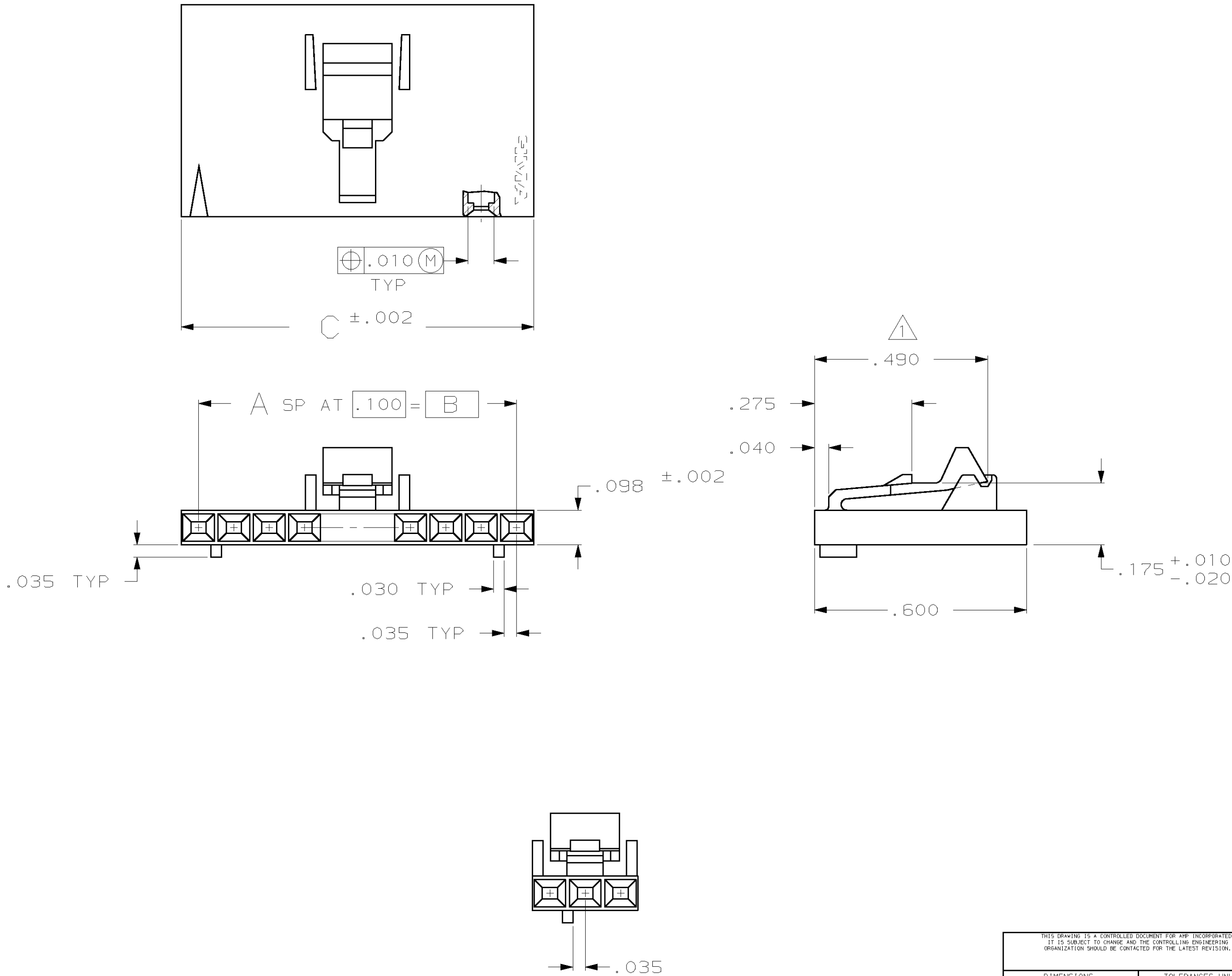
DETAIL FOR -2 ONLY (3 POSITION)
