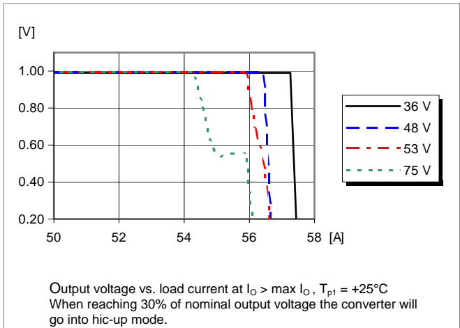
Current Limit Characteristics
