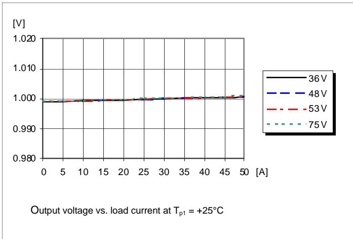
Output Characteristics
